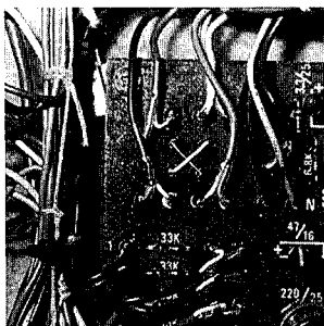
6 – For Echo = PRE, and Foldback = POST, cross jumpers as shown here. Note that at least one of the crossed wires should be insulated to avoid a short-circuit.
