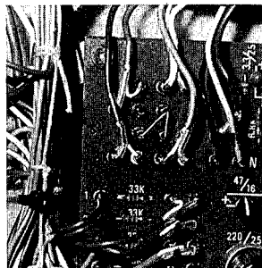
7 – For Echo = POST, and Foldback = POST, connect jumpers as shown here.
